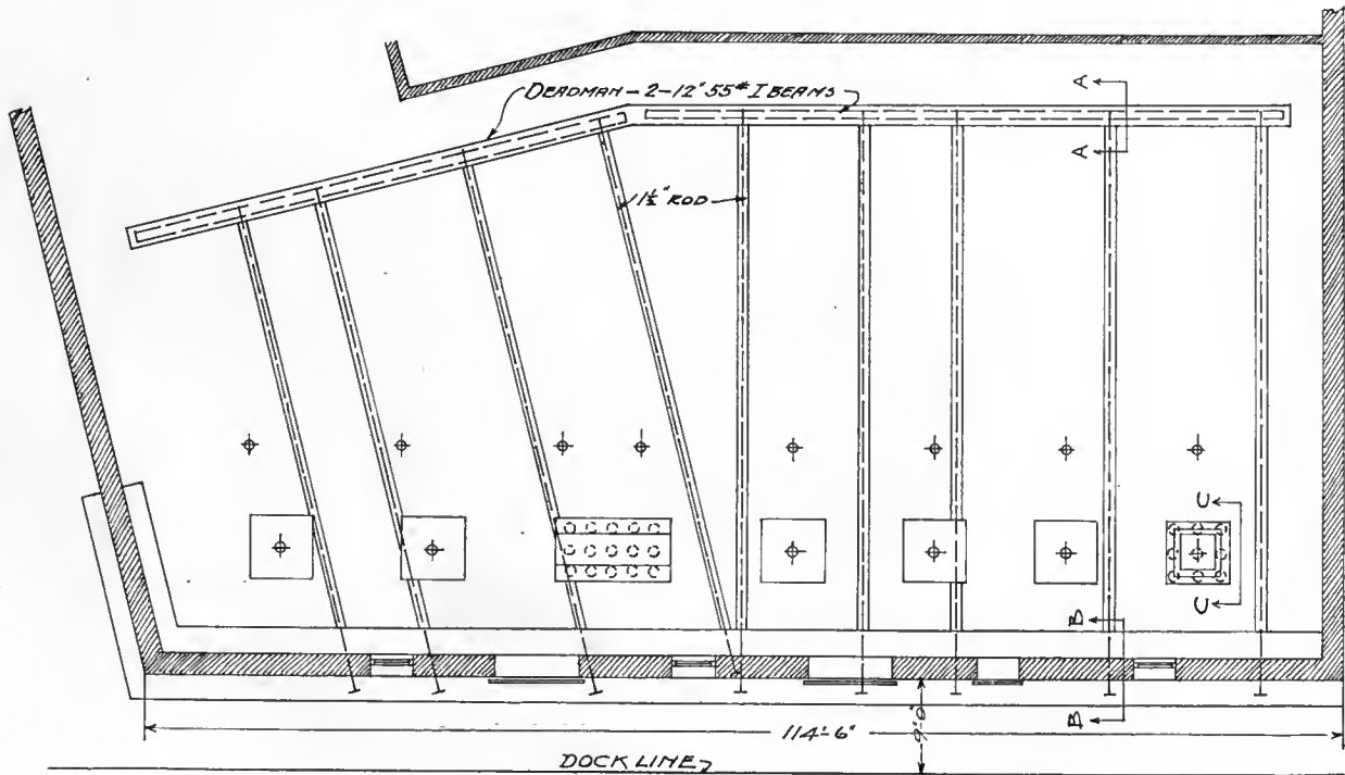
FOUNDATION PLAN
